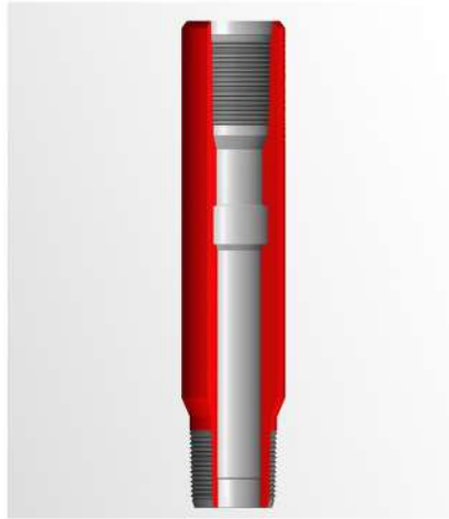
DIC-F Landing Nipples
